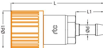
Socket / Kupplung
