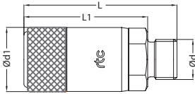
Socket / Kupplung
